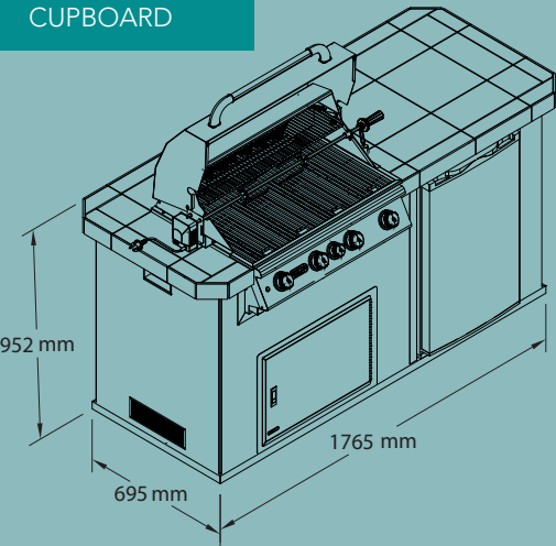
HORIZONTAL CUPBOARD
